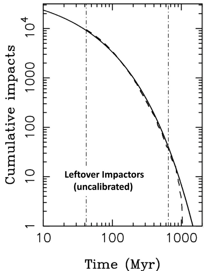
Fig. 8. The (uncalibrated) impact flux of leftover planetesimals on the Earth. The dashed line is the profile for all impacts on the Earth, 9,418 in total, recorded in the simulation after the Moon-forming impact ( t > 42 Myr). The solid line shows the analytic fit given in Eq. (4). The model profile drops more steeply for t = 0.8\text{--}1 Gyr than the analytic fit, because the simulation ended at t = 1 Gyr, and no impacts were recorded for t > 1 Gyr. The vertical dash-dotted lines show t = 42 Myr and t = 650 Myr for reference.
