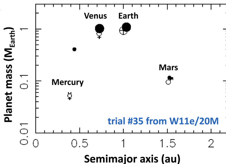
Fig. 1. The mass and radial distribution of terrestrial planets obtained in the best simulation of the W11e/20M model (Nesvorný et al., 2021a). The size of a dot is proportional to the planet mass. The real terrestrial planets are indicated by planetary symbols. The simulation failed to reproduce the correct mass of Mercury, but this is not a major limitation for the present study where we are interested in the impact histories of Venus, Earth, Mars, and the Moon.
