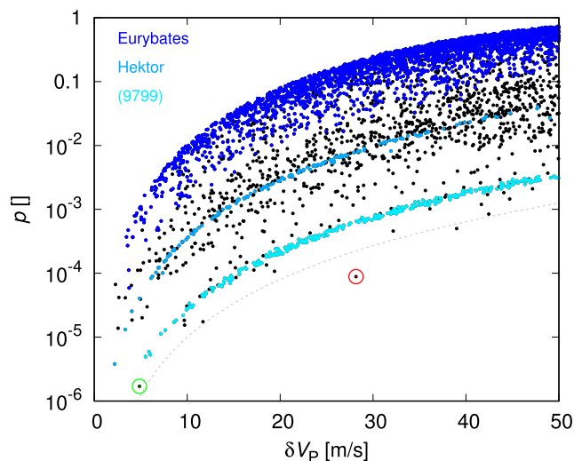
Figure 6. The probability p that a pair is random fluke, computed using the method described in the text, versus its distance \delta V_p , computed for all low-velocity pairs in the L4 zone using equations (2) and (1). The pair (258656) 2002 ES 76 and 2013 CC 41 is highlighted with a red circle. The pair (219902) 2002 EG 134 and (432271) 2009 SH 76 , discussed briefly in Appendix B, is highlighted with a green circle. The coloured symbols denote pairs in the identified L4 families: (i) Eurybates (blue), (ii) the core of the Hektor family (light blue), and (iii) (9799) 1996 RJ (cyan). The dashed line, p = 10^{-5} (\delta V_p / (10 \text{ m s}^{-1}))^3 , is used to emphasize that the candidate pair (258656) 2002 ES 76 and 2013 CC 41 is an outlier in this population.
