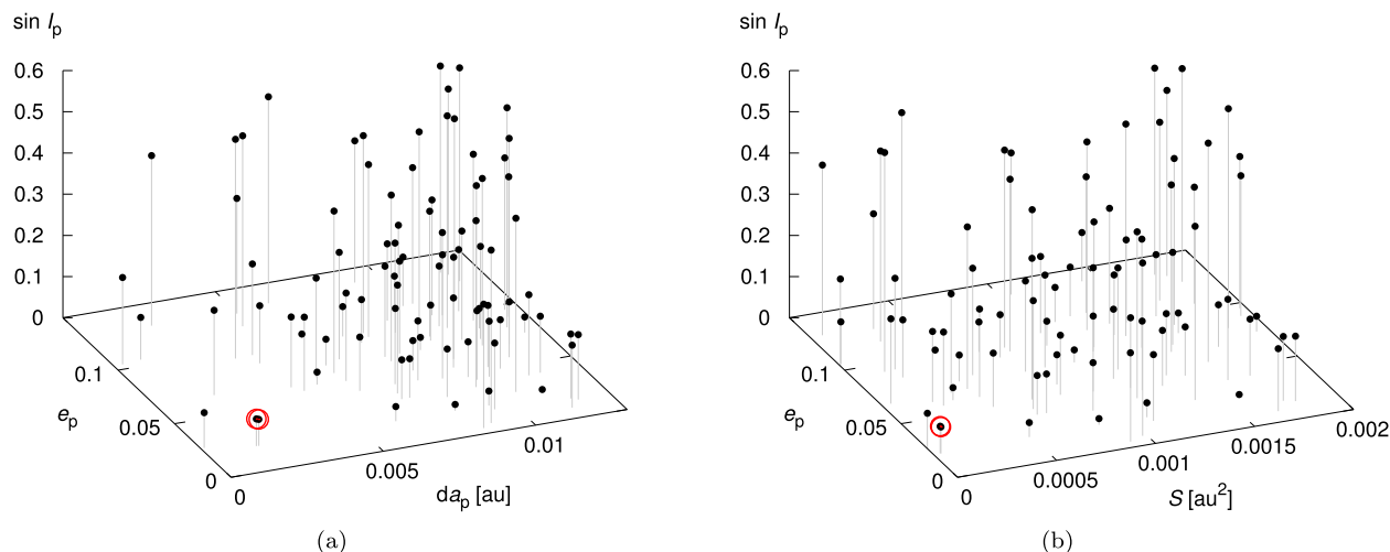
Figure 5. Left-hand panel (a): The small-libration portion of the L4 stable orbital zone in the 3D proper element coordinates ( da_p , e_p , \sin I_p ). The proximity to the libration was arbitrarily set by da_p \leq 0.014 au, whilst the extent of e_p and \sin I_p is limited by orbital stability. We find 91 objects for our data set of Trojans. The candidate pair (258656) 2002 ES 76 and 2013 CC 41 is highlighted with a red circle. The vertical intervals help to appreciate 3D nature of the display. Right-hand panel (b): The same as on the left-hand panel, but the da_p was replaced with a surface area S = 4\pi(da_p)^2 . In this case, the small-amplitude Trojans are distributed more uniformly.
