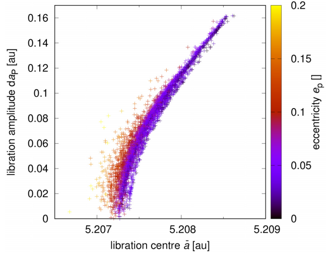
Figure A1. Libration amplitude d_{ap} versus libration centre \bar{a} for Trojans in the L4 region. Colour corresponds to the proper eccentricity e_p . The dependence of \bar{a}(d_{ap}, e_p) is systematic, indicating a functional dependence.
